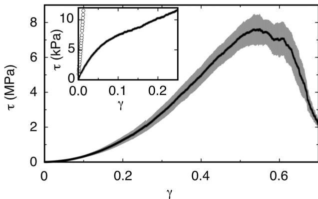
FIG. 2. Stress \tau vs strain \gamma for packings of chains with length N \approx 10^4 . The shaded bands represent 1 standard deviation based on 5 repeated measurements. Strong strain stiffening is seen as the positive curvature in \tau(\gamma) . Inset: \tau(\gamma) for N = 1 (unlinked beads). Open symbols: reproduction of N \approx 10^4 data for comparison on the smaller scale.
