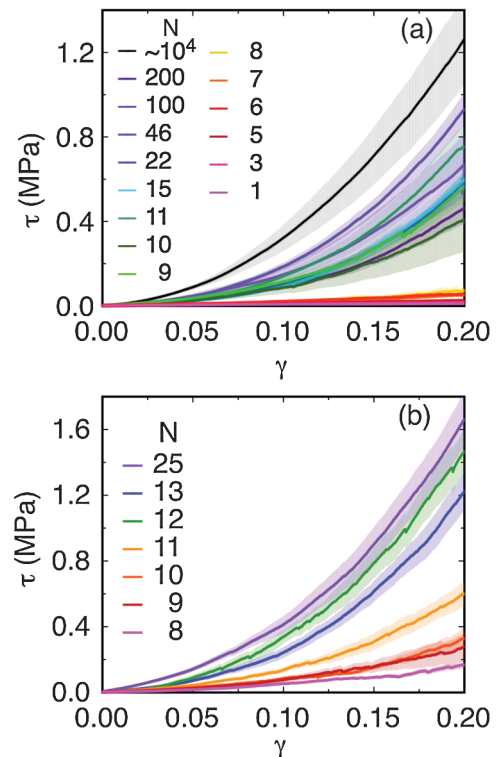
FIG. 3 (color). Stress \tau vs strain \gamma for different chain lengths N shown in the key. (a) For chains of minimum loop circumference \xi = 8 . (b) For \xi = 11 . In both panels, the data for N > \xi (cool colors) group into a band which exhibits strong strain stiffening.
