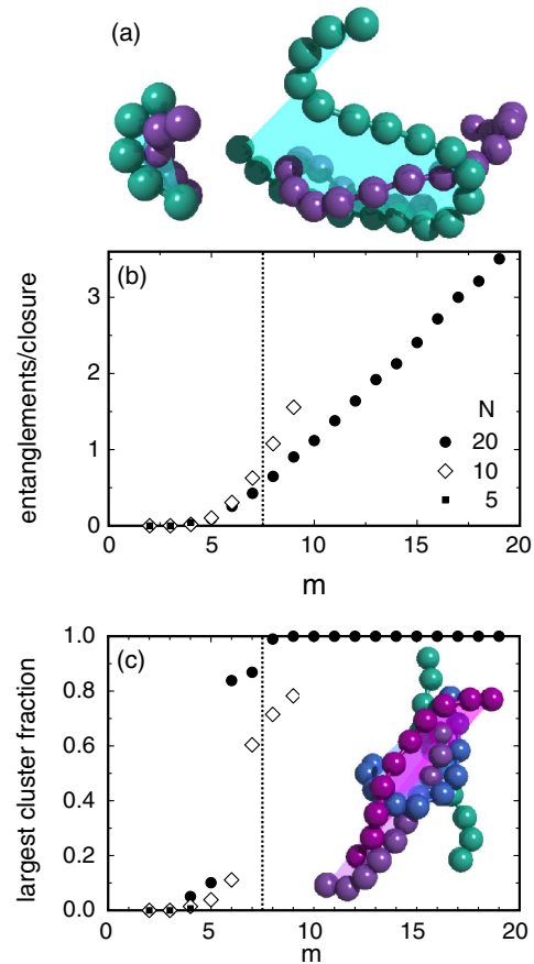
FIG. 4 (color online). (a) Examples of entanglements for chain lengths N = 5 (left) and N = 20 (right). The green chains are entangling the purple chains. The shaded region indicates the entanglement manifold for the closure connecting the ends of the chains ( m = N - 1 ). (b) Average number of entanglements per closure as a function of contour length m for \xi = 8 . The key indicates the chain lengths N . (c) Size of the largest entangled cluster as a fraction of the total number of chains in the sample. The dotted line indicates the onset of strong strain stiffening, which is only found to occur when the contour length of a closure is large enough so that there are entangled clusters consisting of the majority of chains in the system. The inset image shows an example of a cluster of 4 chains with 5 entanglements between them for N = 10 .
