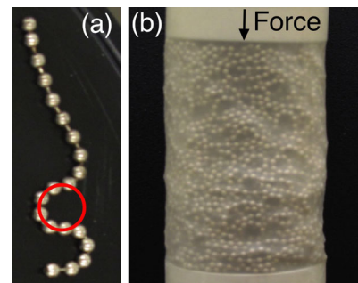
FIG. 1 (color online). (a) An individual chain with length N = 20 beads. The minimum loop size of \xi = 8 beads is highlighted by the red circle. (b) Cylindrical packing of chains with N \gg \xi = 8 inside a thin latex membrane used for uniaxial compression measurements. Many tight loops near the minimum loop size can be seen in the packing through the membrane.
